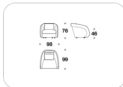
MOL (POLE) EBONY MACASSAR : POLTRONA / ARMCHAIR 98x99x76H. - H.S.46cm 38 2/3x39x30H. - H.S.18"
