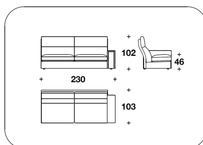
EDE (E3D) - EDE (E3S) ELEMENTO 3 POSTI ALTO DX O SX / 3 SEATER HIGH ELEMENT RIGHT OR LEFT 230x103x102H. - H.S.46cm 90 2/3x40 2/3x40H. - H.S.18"
