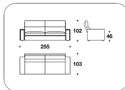
EDE (D3) DIVANO ALTO 3 POSTI / 3 SEATER HIGH SOFA 255x103x102H. - H.S.46cm 100 1/3x40 2/3x40H. - H.S.18"
