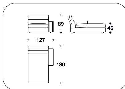
EDE (CLDB) - EDE (CLSB) CHAISE LONGUE : BASSA DESTRA O SINISTRA / LOW RIGHT OR LEFT 127x189x89H. - H.S.46cm 50x74 1/3x35H. - H.S.18"
