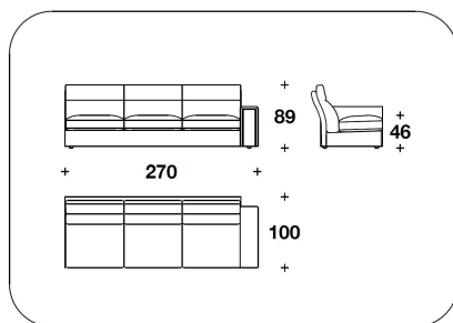
EDE (E4DB) - EDE (E4SB) ELEMENTO 4 POSTI BASSO DX O SX / 4 SEATER LOW ELEMENT RIGHT OR LEFT 270x100x89H. - H.S.46cm 106 1/3x39 1/3x35H. - H.S.18"
