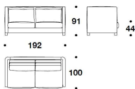
TRU (D2) DIVANO 2 POSTI / 2 SEATER SOFA 192x100x91H. – H.S.44cm 75 2/3x39 1/3x35 2/3H. – H.S.17 1/4"
