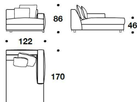
DID (CLDPC) - DID (CLSPC) CHAISE LONGUE CON BRACCIOLO DX O SX / CHAISE LONGUE WITH RIGHT OR LEFT ARM 122x170x86H. – H.S.46cm 48x67x34H. – H.S.18"
