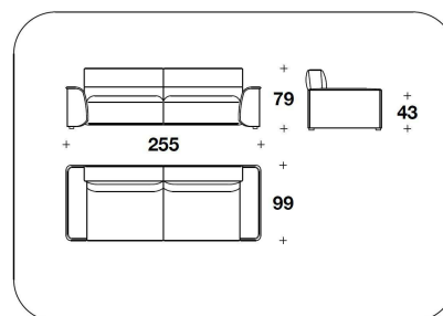
UXB (D3R) CHESTNUT - BURR WALNUT : DIVANO 3 POSTI / 3 SEATER SOFA 255x99x79H. - H.S.43cm 100 1/3x39x31H. - H.S.17"
