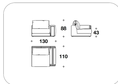
FED (E1DT) - FED (E1ST) ELEMENTO SEDUTA C/BRACCIOLO DX O SX / SEAT ELEMENT W/ARMREST RIGHT OR LEFT 130x110x88H. - H.S.43 cm 51 1/3x43 1/3x34 2/3H. - H.S.17 "
