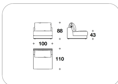
FED (E1CNT) ELEMENTO SEDUTA SENZA BRACCIOLO / SEAT ELEMENT WITHOUT ARMREST 100x110x88H. - H.S.43 cm 39 1/3x43 1/3x34 2/3H. - H.S.17 "
