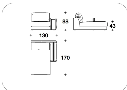
FED (CLDT) - FED (CLST) CHAISE LONGUE : ELEMENTO SEDUTA DX O SX / SEAT ELEMENT RIGHT OR LEFT 130x170x88H. - H.S.43 cm 51 1/3x67x34 2/3H. - H.S.17 "
