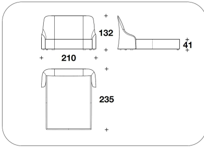
AUD (LE1) LETTO PER MATERASSO CON RETROTESTIERA IN FODERA / BED FOR MATTRESS WITH LINING BACK HEADBOARD 165x200 210x235x132H. - H.B.41cm 65x78 2/3 82 2/3x92 2/3x52H. - H.B.16 1/4"
