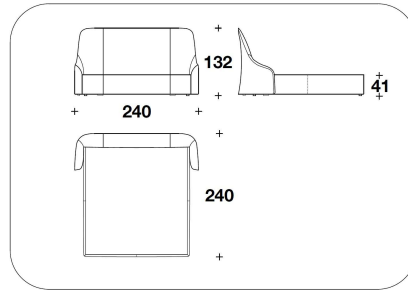
AUD (KUSA) KING USA : LETTO PER MATERASSO CON RETROTESTIERA IN FODERA / BED FOR MATTRESS WITH LINING BACK HEADBOARD 195x205 240x240x132H. - H.B.41cm 76 2/3x80 2/3 94 1/3x94 1/3x52H. - H.B.16 1/4"
