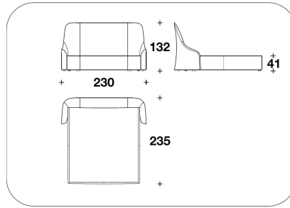
AUD (LE2) LETTO PER MATERASSO CON RETROTESTIERA IN FODERA / BED FOR MATTRESS WITH LINING BACK HEADBOARD 185x200 230x235x132H. - H.B.41cm 73x78 2/3 90 2/3x92 2/3x52H. - H.B.16 1/4"
