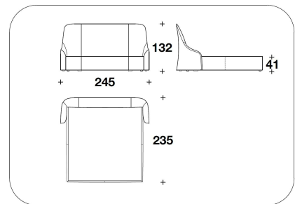
AUD (ALE7) LETTO PER MATERASSO / BED FOR MATTRESS 200x200 245x235x132H. - H.B.41cm 78 2/3x78 2/3 96 1/3x92 2/3x52H. - H.B.16 1/4"
