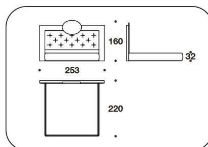
CEO (ALE7) LETTO PER MATERASSO / BED FOR MATTRESS 200x200 - 253x220x160H. - H.B.32 cm 78 2/3x78 2/3 - 99 2/3x86 2/3x63H. - H.B.12 2/4 "
