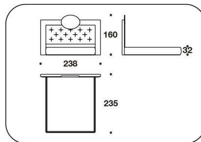
CEO (ACUSA) CALIFORNIA USA : LETTO PER MATERASSO / BED FOR MATTRESS 183x215 - 238x235x160H. - H.B.32 cm 72x84 2/3 - 93 2/3x92 2/3x63H. - H.B.12 2/4 "
