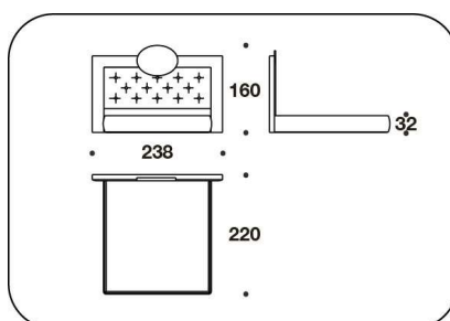
CEO (ALE2) LETTO PER MATERASSO / BED FOR MATTRESS 185x200 - 238x220x160H. - H.B.32 cm 73x78 2/3 - 93 2/3x86 2/3x63H. - H.B.12 2/4 "
