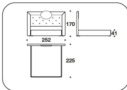
CEO (MKUSA) KING USA : LETTO PER MATERASSO / BED FOR MATTRESS 195x205 - 252x225x170H. - H.B.41cm 76 2/3x80 2/3 - 99 1/3x88 2/3x67H. - H.B.16 1/4"
