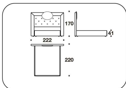
CEO (MLE1) LETTO PER MATERASSO / BED FOR MATTRESS 165x200 - 222x220x170H. - H.B.41cm 65x78 2/3 - 87 1/3x86 2/3x67H. - H.B.16 1/4"
