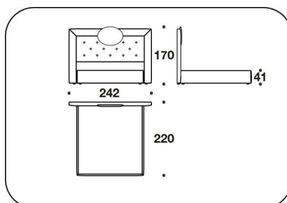
CEO (MLE2) LETTO PER MATERASSO / BED FOR MATTRESS 185x200 - 242x220x170H. - H.B.41cm 73x78 2/3 - 95 1/3x86 2/3x67H. - H.B.16 1/4"
