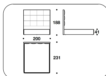
DMN (CUSAI) CALIFORNIA USA : LETTO PER MATERASSO / BED FOR MATTRESS 183x215 - 200x231x188H. - H.B.41 cm 72x84 2/3 - 78 2/3x91x74H. - H.B.16 1/4 "
