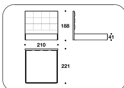
DMN (KUSAI) KING USA : LETTO PER MATERASSO / BED FOR MATTRESS 195x205 - 210x221x188H. - H.B.41 cm 76 2/3x80 2/3 - 82 2/3x87x74H. - H.B.16 1/4 "
