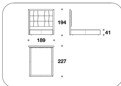
SM2 (QUSA) QUEEN USA : LETTO PER MATERASSO / BED FOR MATTRESS 152x205 - 189x227x194H. - H.B.41cm 60x80 2/3 - 74 1/3x89 1/3x76 1/3H. - H.B.16 1/4"
