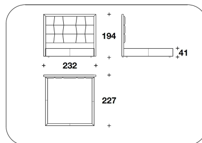
SM2 (KUSA) KING USA : LETTO PER MATERASSO / BED FOR MATTRESS 195x205 - 232x227x194H. - H.B.41cm 76 2/3x80 2/3 - 91 1/3x89 1/3x76 1/3H. - H.B.16 1/4"
