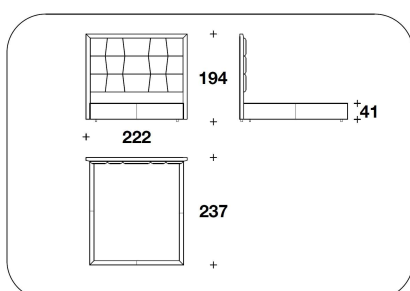
SM2 (CUSA) CALIFORNIA USA : LETTO PER MATERASSO / BED FOR MATTRESS 183x215 - 222x237x194H. - H.B.41cm 72x84 2/3 - 87 1/3x93 1/3x76 1/3H. - H.B.16 1/4"
