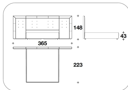
NRF (AKUSA) KING USA : LETTO PER MATERASSO CON SPONDE LATERALI / BED FOR MATTRESS WITH LATERAL SIDES 195x205 365x223x148H. - H.B.43cm 76 2/3x80 2/3 143 1/2x87 2/3x58 1/3H. - H.B.17"
