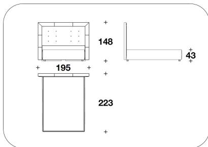
NRF (QUSA) QUEEN USA : LETTO PER MATERASSO / BED FOR MATTRESS 152x205 195x223x148H. - H.B.43cm 60x80 2/3 76 2/3x87 2/3x58 1/3H. - H.B.17"
