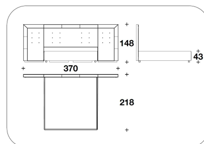
NRF (ALE7) LETTO PER MATERASSO CON SPONDE LATERALI / BED FOR MATTRESS WITH LATERAL SIDES 200x200 370x218x148H. - H.B.43cm 78 2/3x78 2/3 145 1/2x85 2/3x58 1/3H. - H.B.17"
