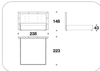
NRF (KUSA) KING USA : LETTO PER MATERASSO / BED FOR MATTRESS 195x205 238x223x148H. - H.B.43cm 76 2/3x80 2/3 93 2/3x87 2/3x58 1/3H. - H.B.17"
