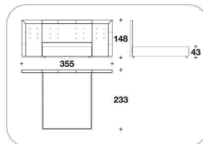
NRF (ACUSA) CALIFORNIA USA : LETTO PER MATERASSO CON SPONDE LATERALI / BED FOR MATTRESS WITH LATERAL SIDES 183x215 355x233x148H. - H.B.43cm 72x84 2/3 140x91 2/3x58 1/3H. - H.B.17"
