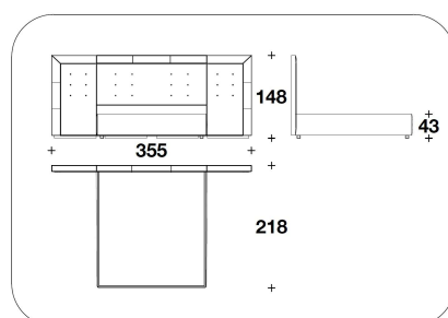
NRF (ALE2) LETTO PER MATERASSO CON SPONDE LATERALI / BED FOR MATTRESS WITH LATERAL SIDES 185x200 355x218x148H. - H.B.43cm 73x78 2/3 140x85 2/3x58 1/3H. - H.B.17"
