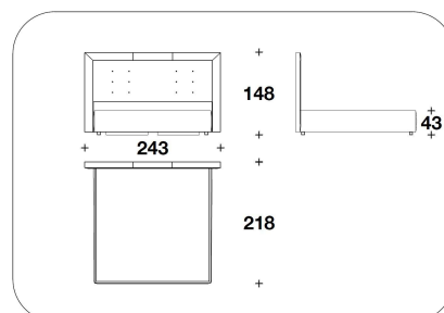
NRF (LE7) LETTO PER MATERASSO / BED FOR MATTRESS 200x200 243x218x148H. - H.B.43cm 78 2/3x78 2/3 95 2/3x85 2/3x58 1/3H. - H.B.17"
