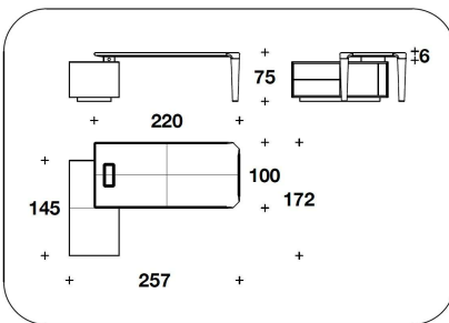
TAV (T97EE1) - TAV (T97EE3) EBONY MACASSAR : SCRIVANIA DX O SX / RIGHT OR LEFT WRITING-DESK L.220 (257x172/217)x75H.cm L.86 2/3 (101 1/3x67 2/3/85 1/3)x29 2/3H."
