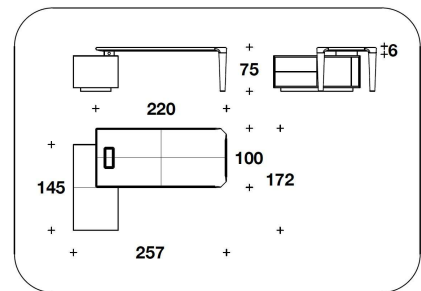
TAV (T97PMP1) - TAV (T97PMP3) - TAV (T97PPP1) - TAV (T97PPP3) LEATHER : SCRIVANIA DX O SX / RIGHT OR LEFT WRITING-DESK L.220 (257x172/217)x75H.cm L.86 2/3 (101 1/3x67 2/3/85 1/3)x29 2/3H."
