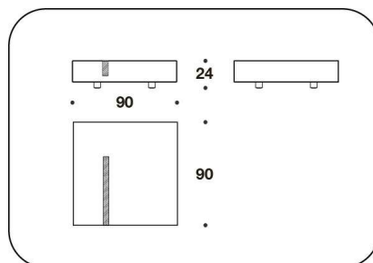
TCT (CA19P) - TCT (CA19E) COFFEE TABLE 90x90x24H.cm 35 1/3x35 1/3x9 2/4H."
