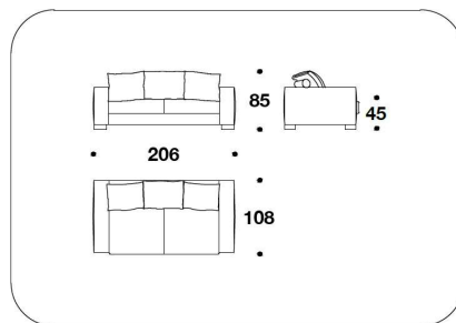
A2E (D2) DIVANO 2 POSTI / 2 SEATER SOFA 206x108x85H. - H.S.45cm 81x42 2/3x33 1/3H. - H.S.17 3/4"
