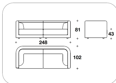
ER1 (D3) DIVANO 3 POSTI / 3 SEATER SOFA 248x102x81H. - H.S.43cm 97 2/3x40x32H. - H.S.17"
