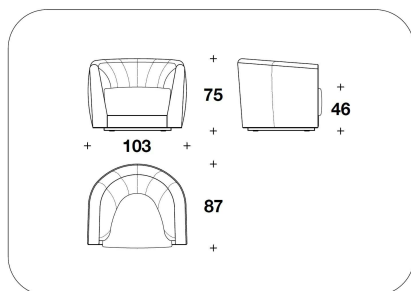
POF (15) POLTRONA / ARMCHAIR 103x87x75H. - H.S.46 cm 40 2/3x34 1/3x29 2/3H. - H.S.18 "
