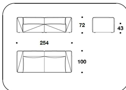
DGN (D3) DIVANO 3 POSTI / 3 SEATER SOFA 254x100x72H. - H.S.43cm 100x39 1/3x28 1/3H. - H.S.17"
