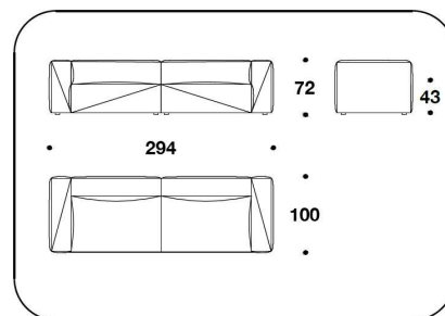
DGN (D4) DIVANO 4 POSTI / 4 SEATER SOFA 294x100x72H. - H.S.43cm 115 2/3x39 1/3x28 1/3H. - H.S.17"
