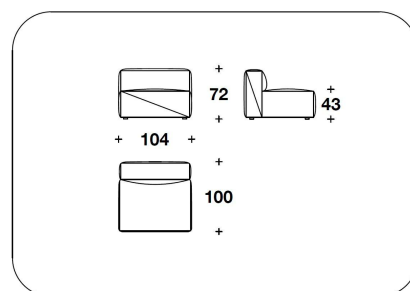
DGN (E1CNP) ELEMENTO CENTRALE PICCOLO / SMALL CENTRAL ELEMENT 104x100x72H. - H.S.43cm 41x39 1/3x28 1/3H. - H.S.17"
