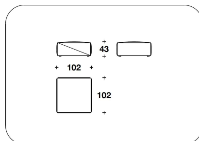
DGN (POU) POUF / OTTOMAN 102x102x43H.cm 40x40x17H."
