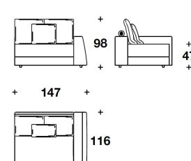
ELN (AE1D) - ELN (AE1S) ELEMENTO 1 POSTO CON BRACCIOLO DX O SX / 1 SEATER ELEMENT WITH RIGHT OR LEFT ARMREST 147x116x98H. - H.S.47cm 58x45 2/3x38 2/3H. - H.S.18 2/4"
