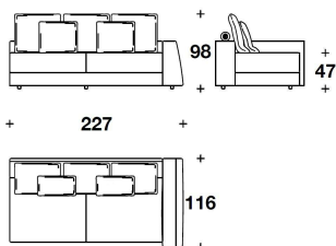
ELN (AE2D) - ELN (AE2S) ELEMENTO 2 POSTI CON BRACCIOLO DX O SX / 2 SEATER ELEMENT WITH RIGHT OR LEFT ARMREST 227x116x98H. - H.S.47cm 89 1/3x45 2/3x38 2/3H. - H.S.18 2/4"
