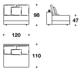
ELN (AE1C) ELEMENTO CENTRALE 1 POSTO / 1 SEATER CENTRAL ELEMENT 120x110x98H. - H.S.47 cm 47 1/3x43 1/3x38 2/3H. - H.S.18 2/4 "
