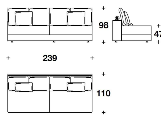
ELN (AE4C) ELEMENTO CENTRALE 4 POSTI / 4 SEATER CENTRAL ELEMENT 240x110x98H. - H.S.47 cm 94 1/3x43 1/3x38 2/3H. - H.S.18 2/4 "
