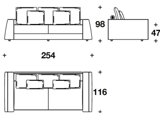
ELN (AD2) DIVANO 2 POSTI / 2 SEATER SOFA 254x116x98H. - H.S.47cm 100x45 2/3x38 2/3H. - H.S.18 2/4"
