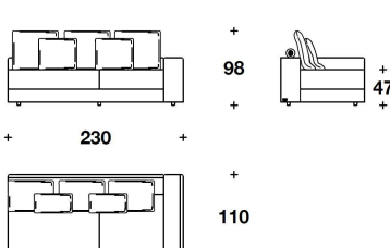
ELN (AE1AD) - ELN (AE1AS) ELEMENTO ANGOLARE 1 POSTO DX O SX / 1 SEATER CORNER ELEMENT RIGHT OR LEFT 230x110x98H. - H.S.47 cm 90 2/3x43 1/3x38 2/3H. - H.S.18 2/4 "
