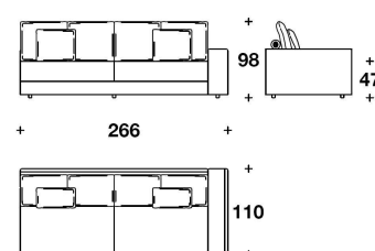
ELN (AE4AD) - ELN (AE4AS) ELEMENTO ANGOLARE 4 POSTI DX O SX / 4 SEATER CORNER ELEMENT RIGHT OR LEFT 266x110x98H. - H.S.47 cm 104 2/3x43 1/3x38 2/3H. - H.S.18 2/4 "
