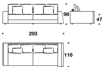
ELN (AD4AD) - ELN (AD4AS) DIVANO ANGOLARE 4 POSTI CON BRACCIOLO DX O SX / 4 SEATER CORNER SOFA WITH RIGHT OR LEFT ARM 293x116x98H. - H.S.47cm 115 1/3x45 2/3x38 2/3H. - H.S.18 2/4"
