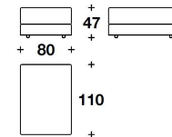
ELN (POUR) POUF RETTANGOLARE / RECTANGULAR OTTOMAN 80x110x47H.cm 31 1/3x43 1/3x18 2/4H."
