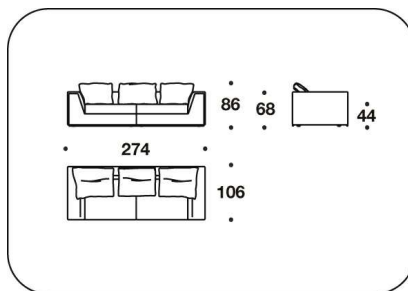
DFE (D3) DIVANO 3 POSTI / 3 SEATER SOFA 274x106x86H. - H.S.44cm 108x41 2/3x34H. - H.S.17 1/4"
