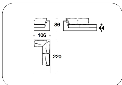
DFE (MED) - DFE (MES) MERIDIENNE DX O SX / RIGHT OR LEFT 106x220x86H. - H.S.44cm 41 2/3x86 2/3x34H. - H.S.17 1/4"
