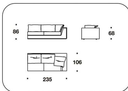
DFE (E3D) - DFE (E3S) ELEMENTO 3 POSTI CON BRACCIO DX O SX / 3 SEATER ELEMENT WITH ARM RIGHT OR LEFT 235x106x86H. - H.S.44cm 92 2/3x41 2/3x34H. - H.S.17 1/4"
