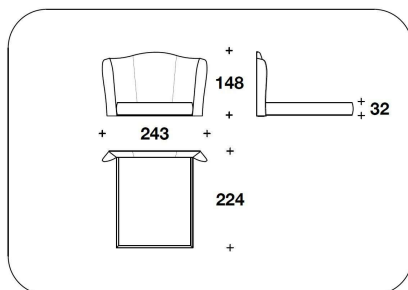
JOL (LE1) LETTO PER MATERASSO / BED FOR MATTRESS 165x200 - 243x224x148H. - H.B.32cm 65x78 2/3 - 95 2/3x88 1/3x58 1/3H. - H.B.12 2/4"
