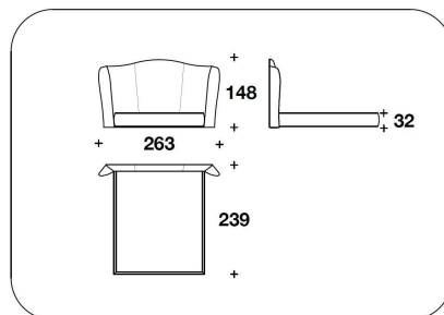
JOL (CUSA) CALIFORNIA USA : LETTO PER MATERASSO / BED FOR MATTRESS 183x215 - 263x239x148H. - H.B.32cm 72x84 2/3 - 103 2/3x94x58 1/3H. - H.B.12 2/4"
