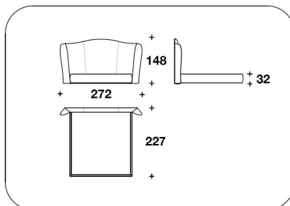
JOL (KUSA) KING USA : LETTO PER MATERASSO / BED FOR MATTRESS 195x205 - 272x227x148H. - H.B.32cm 76 2/3x80 2/3 - 107x89 1/3x58 1/3H. - H.B.12 2/4"
