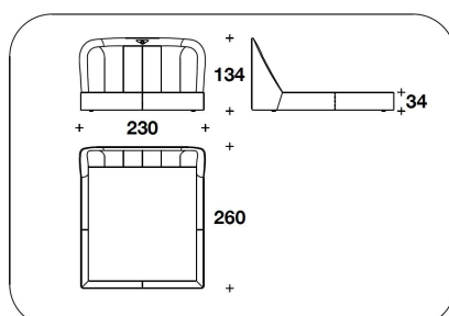
BEL (KUSA) KING USA : LETTO PER MATERASSO / BED FOR MATTRESS 195x205 - 230x260x134H. - H.B.34cm 76 2/3x80 2/3 - 90 2/3x102 1/3x52 2/3H. - H.B.13 2"
