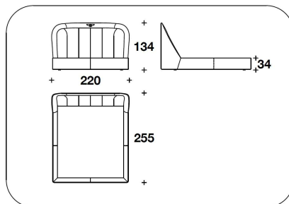
BEL (LE2) LETTO PER MATERASSO / BED FOR MATTRESS 185x200 - 220x255x134H. - H.B.34cm 73x78 2/3 - 86 2/3x100 1/3x52 2/3H. - H.B.13 2/4"
