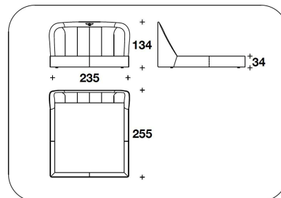
BEL (LE7) LETTO PER MATERASSO / BED FOR MATTRESS 200x200 - 235x255x134H. - H.B.34cm 78 2/3x78 2/3 - 92 2/3x100 1/3x52 2/3H. - H.B.13 2"
