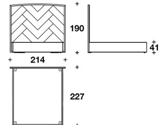
CVR (CUSAE) - CVR (CUSAL) CALIFORNIA USA : LETTO PER MATERASSO / BED FOR MATTRESS 183x215 - 214x227x190H. - H.B.41cm 72x84 2/3 - 84 1/3x89 1/3x74 2/3H. - H.B.16 1/4"
