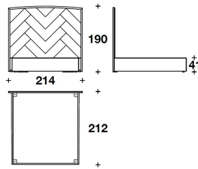
CVR (LE2E) - CVR (LE2L) LETTO PER MATERASSO / BED FOR MATTRESS 185x200 - 214x212x190H. - H.B.41cm 73x78 2/3 - 84 1/3x83 1/3x74 2/3H. - H.B.16 1/4"
