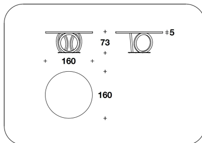
TAV (T66L) - TAV (T66P) - TAV (T66E) - TAV (T66R) - TAV (T66PA) TAVOLO ROTONDO / ROUND TABLE Ø 160x73H. - THK.5cm Ø 63x28 2/3H. - THK.1 15/16"
