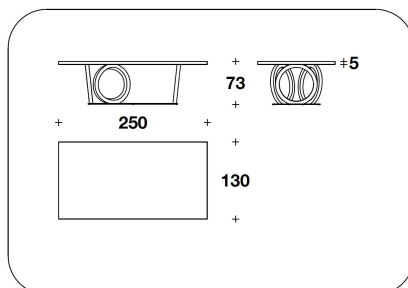
TAV (T68L) - TAV (T68P) - TAV (T68E) - TAV (T68R) - TAV (T68PA) TAVOLO RETTANGOLARE / RECTANGULAR TABLE 250x130x73H. - THK.5cm 98 1/3x51 1/3x28 2/3H. - THK.1 15/16"
